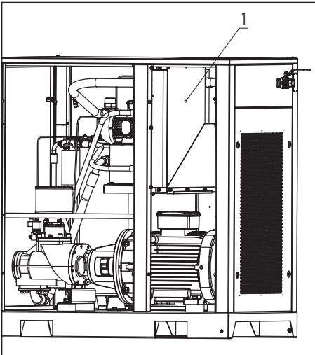
Fig. 5.6 Cleaning radiator
