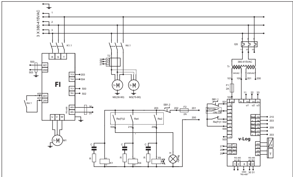
Fig. 2.6 Electrical diagram DV30-55
