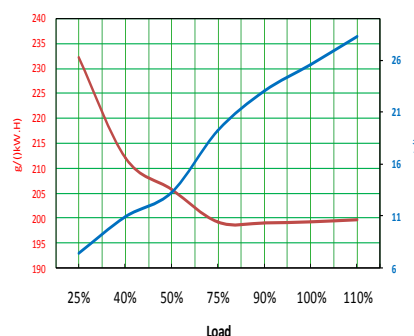
4M11G90/6e2-108kW/1800rpm
